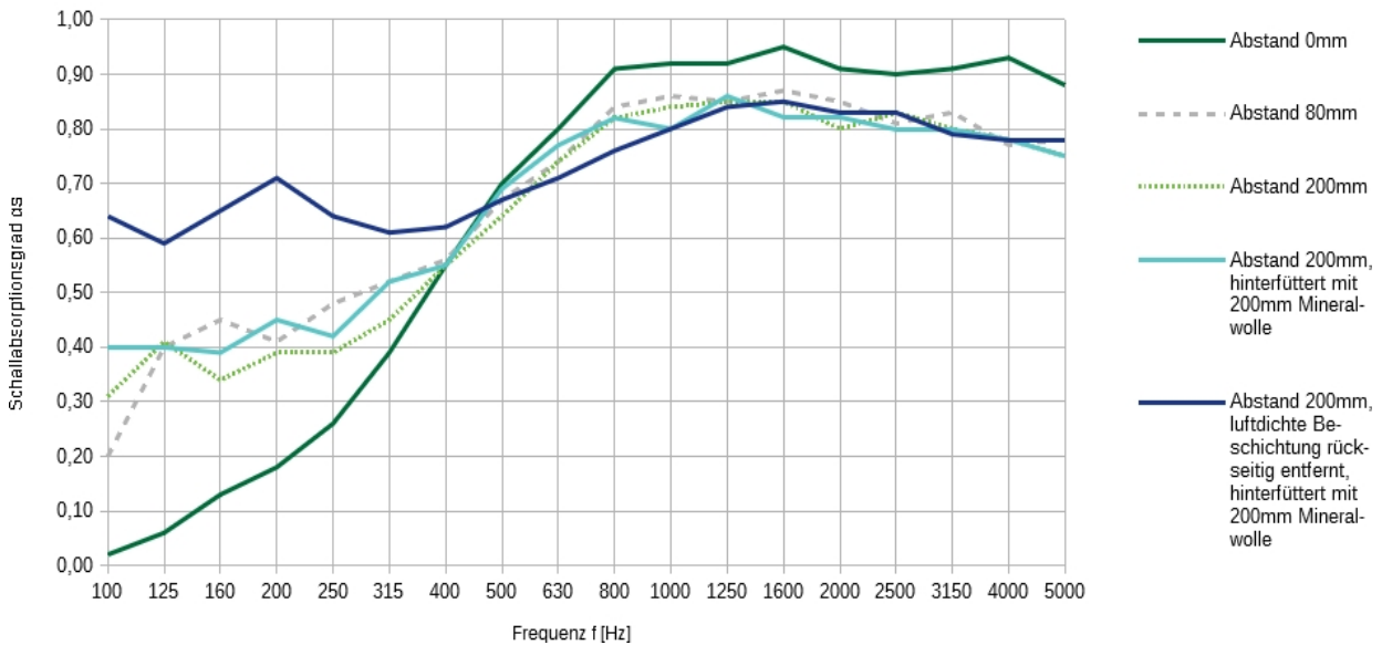
Schallabsorptionsgrade DISTANCE-Easy
